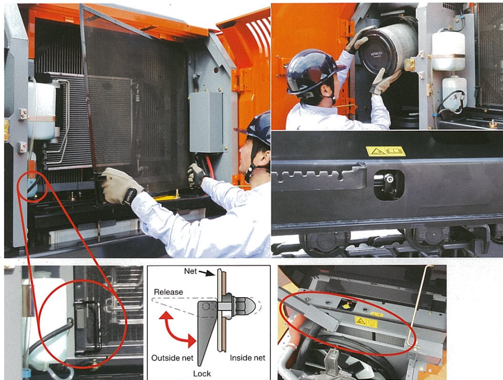
One-touch Openable Upper Cover
